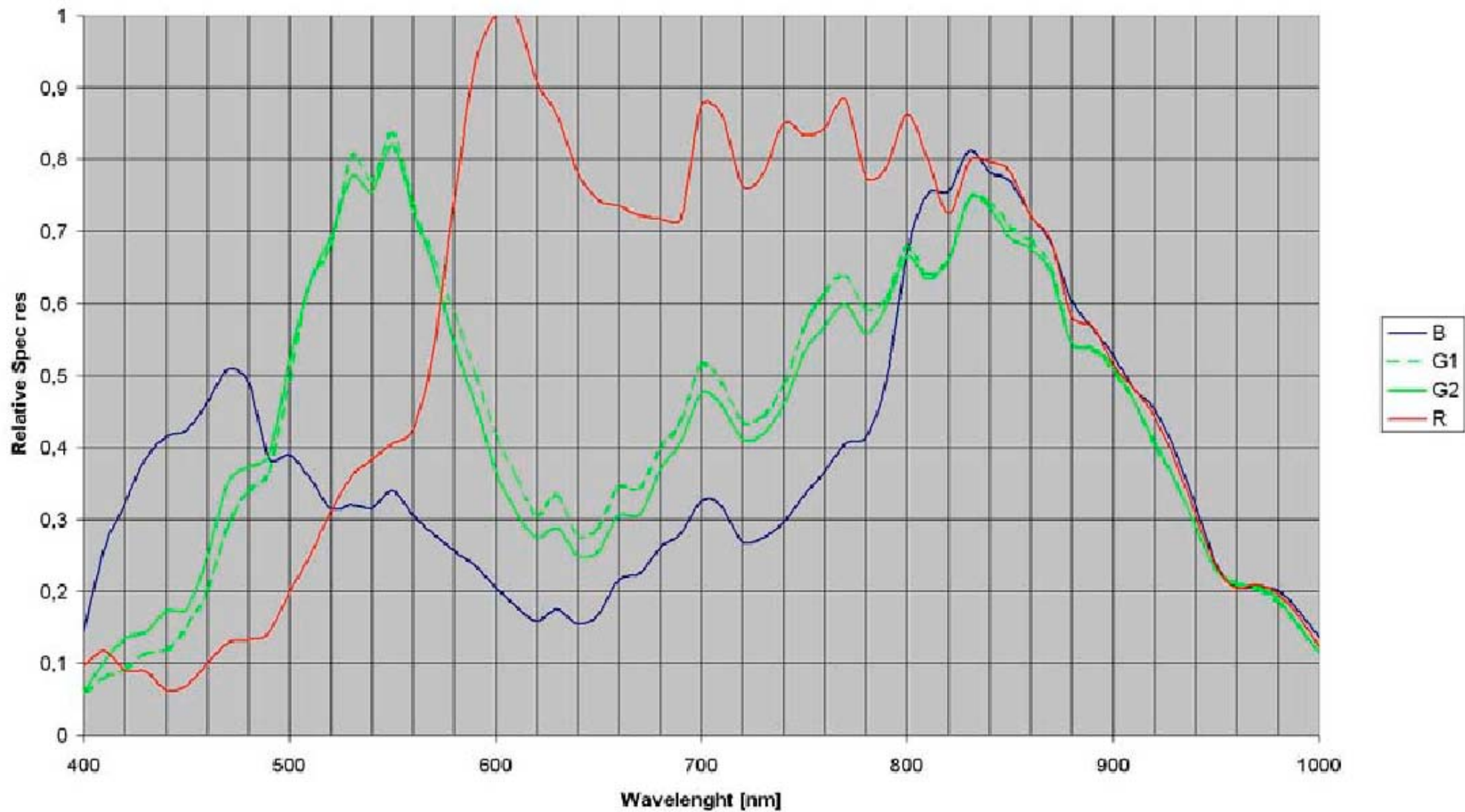
IBIS5A Colour Filter Spectral Response
