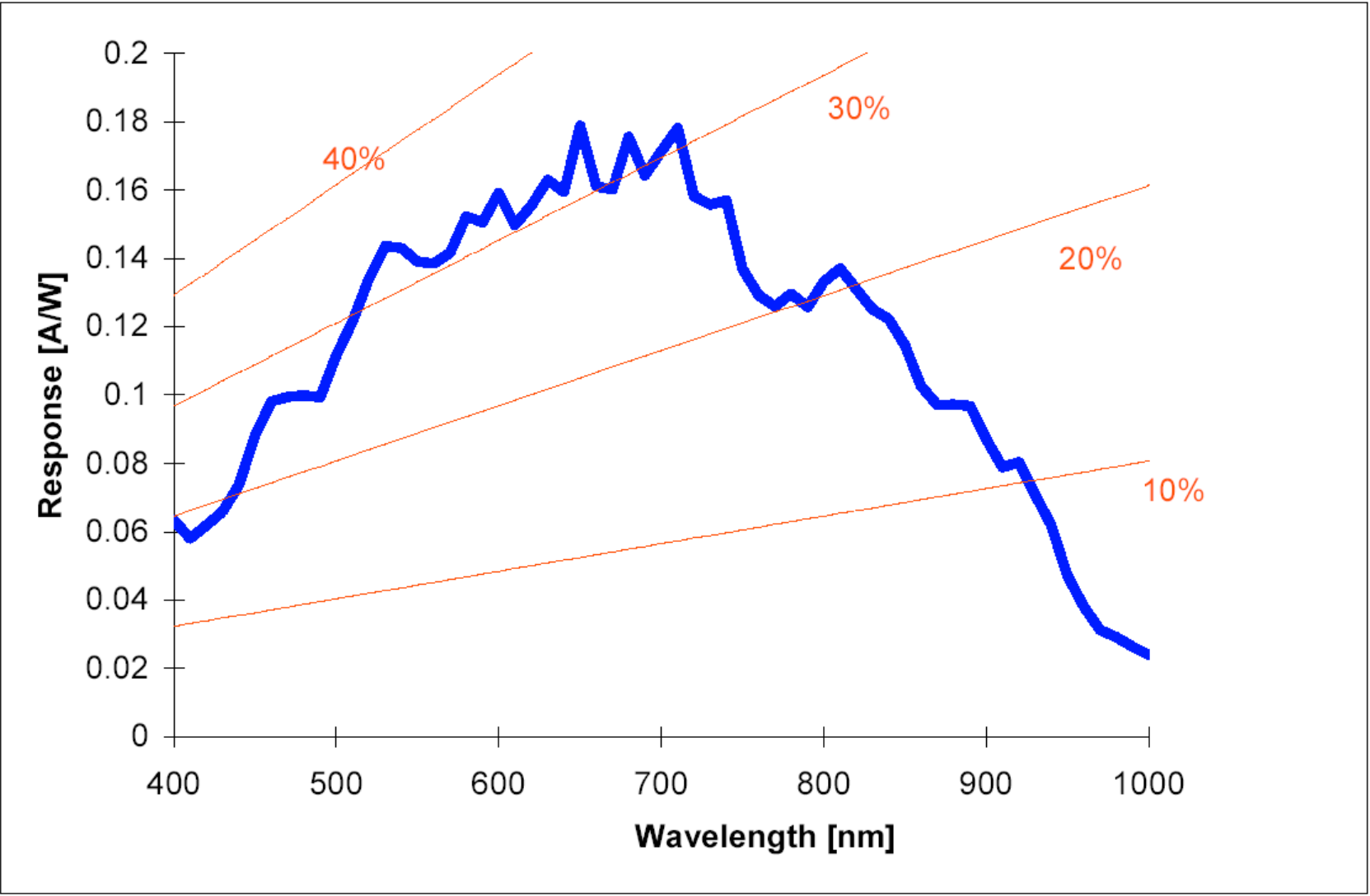
IBIS4-1300 Spectral Response * Fill-Factor
